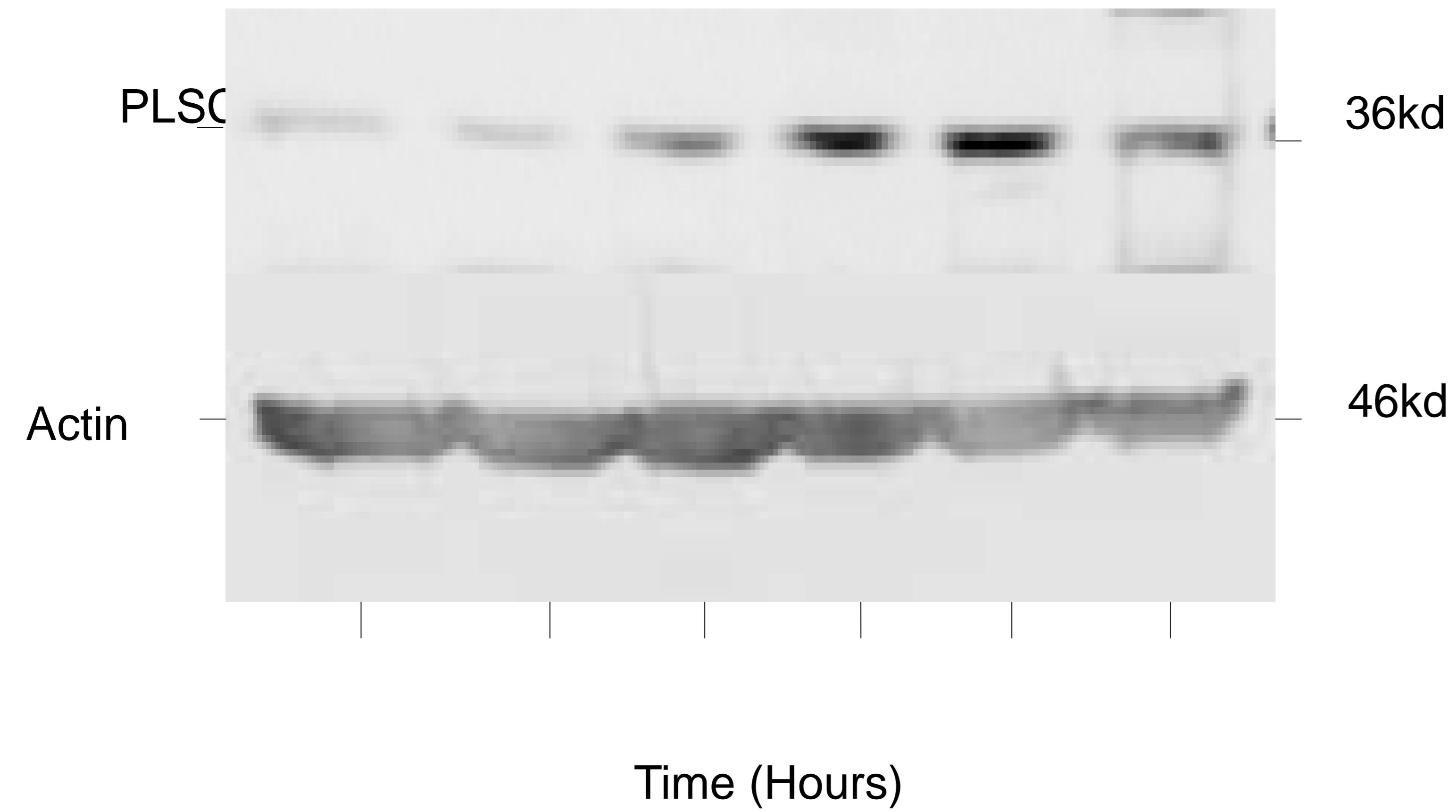
Western Blot
